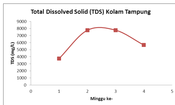
Gambar 4. Monitoring TDS Air Lindi Kolam Tampung
