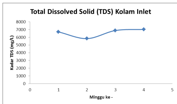
Gambar 1. Monitoring TDS Air Lindi Inlet
