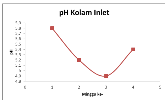
Gambar 3. Monitoring pH Air Lindi Inlet
