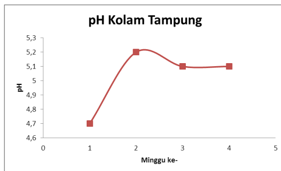
Gambar 6. Monitoring pH Air Lindi Kolam Tampung
