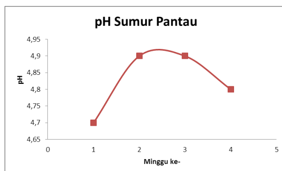
Gambar 9. Monitoring pH Air Sumur Pantau
