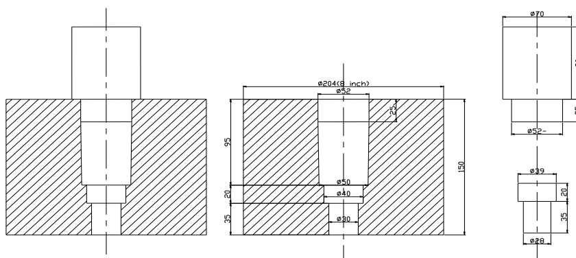
Gambar 1. Disain die-punch
