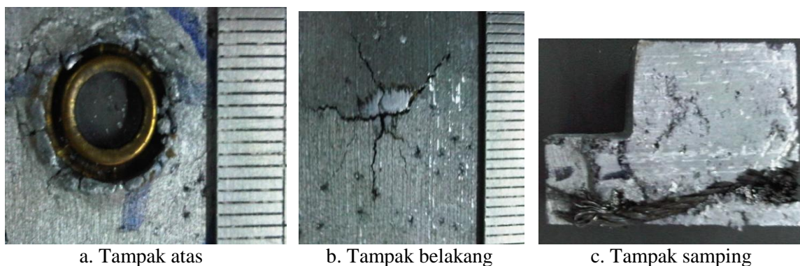
Gambar 5. Hasil Uji Tembak ( Ballistic test )
