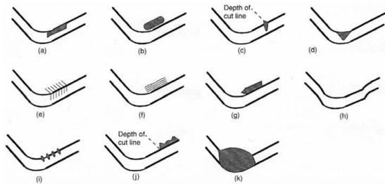
Gambar 1. Macam-macam Keausan Pahat [18]
