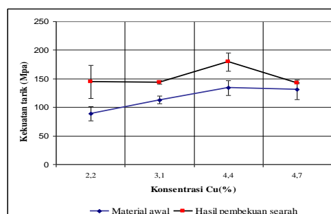
Gambar 1.11 Hasil uji tarik paduan Al-Cu
